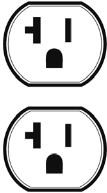
Figure 1. NEMA 5-20R: 125 Volt, 20 Amp Duplex Receptacle
