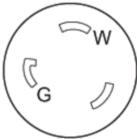
Figure 2. L5-30R: 120Volt, 30Amp Twist Lock Receptacle
